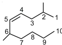
2, 6-Dimethyldec-4-ene
